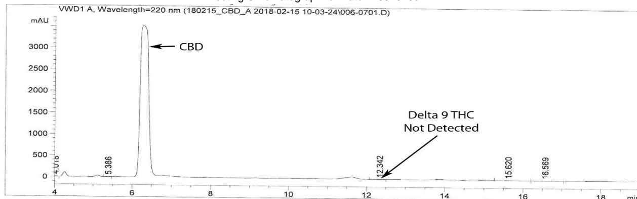
Testing Chromatograph for Batch 20816209
